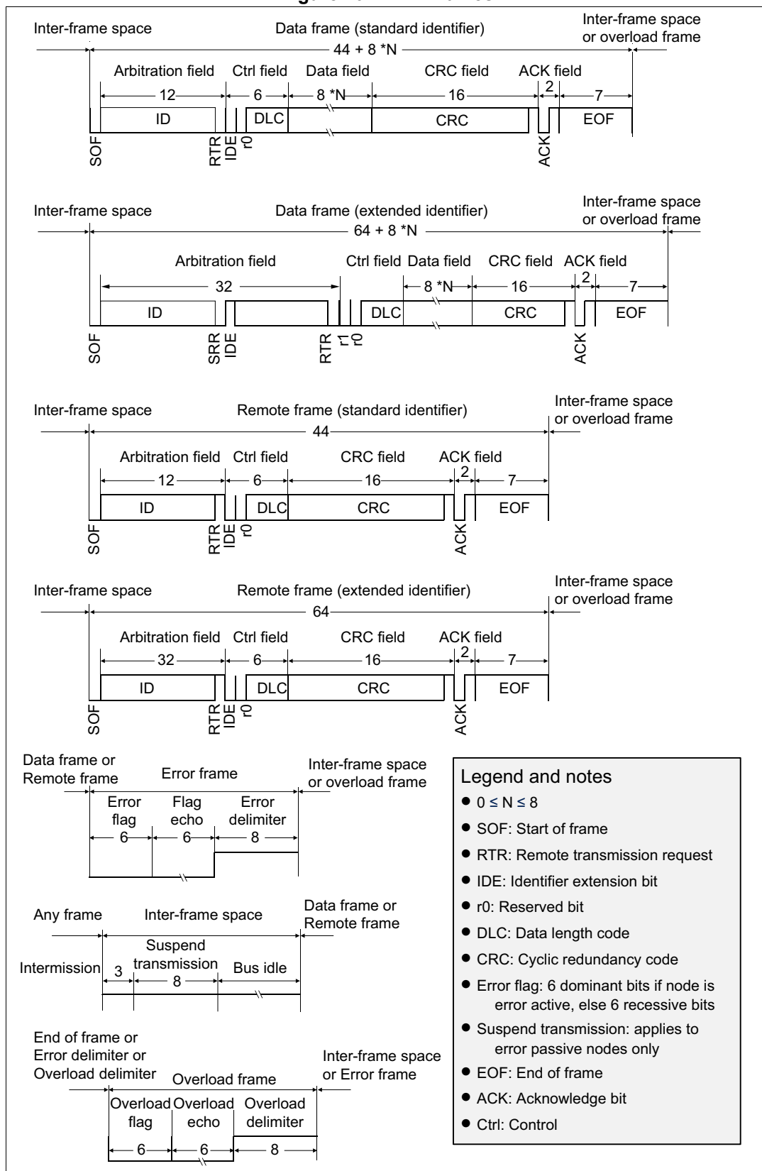
Figure 401. CAN frames
