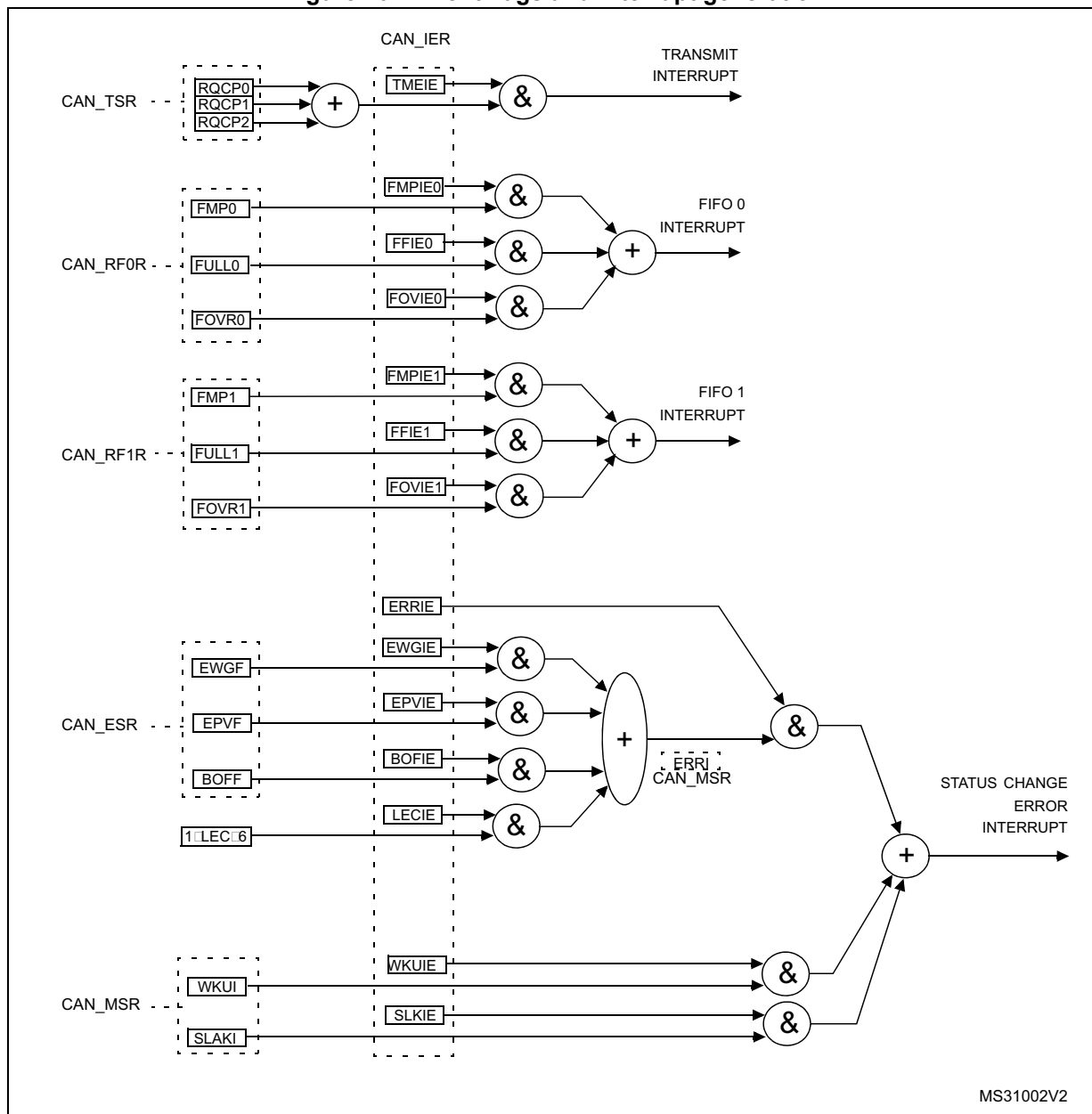
Figure 402. Event flags and interrupt generation
