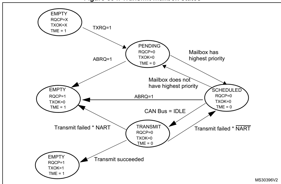
Figure 394. Transmit mailbox states
